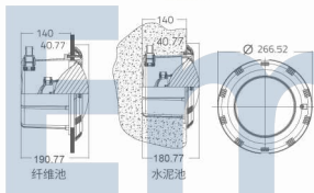
型号: LED P300
