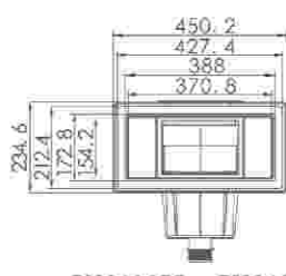
EM01405C EM01405V
