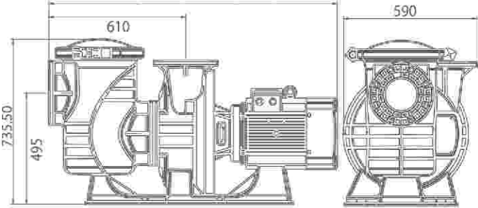
APS1000P/APS1500P
